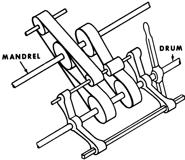
Figure 8-6. Belt-pulley feed works.
